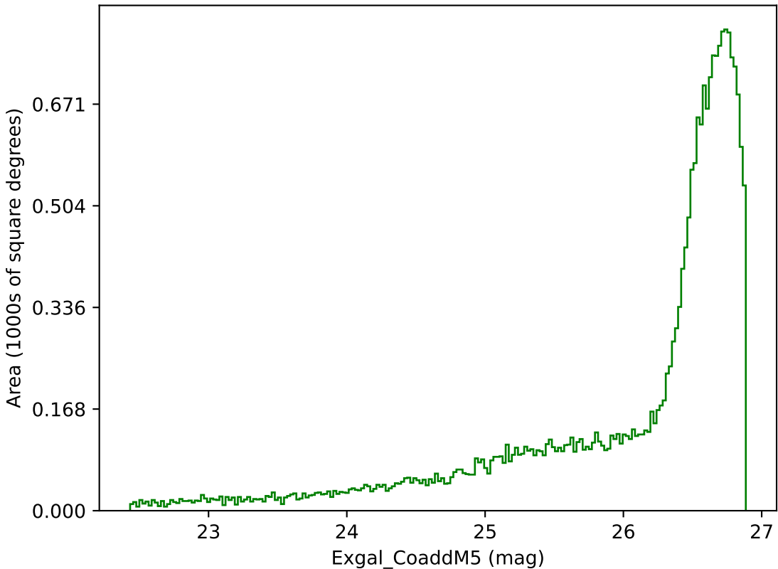
weather_cloudso10v3.4_10yrs All sky g band: Exgal_CoaddM5
