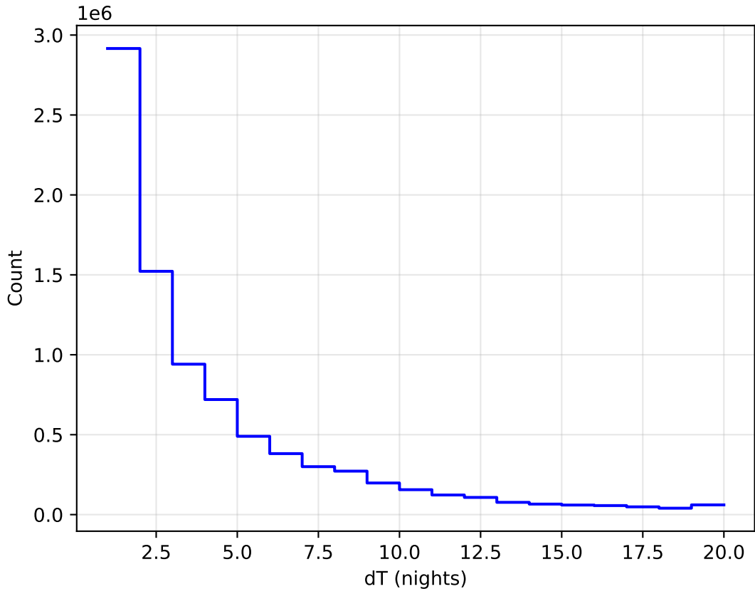
weather_cloudso10v3.4_10yrs WFD all bands: DeltaNight Histogram
