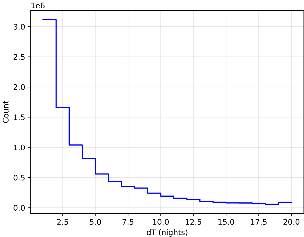
weather_cloudso10v3.4_10yrs All sky all bands: DeltaNight Histogram
