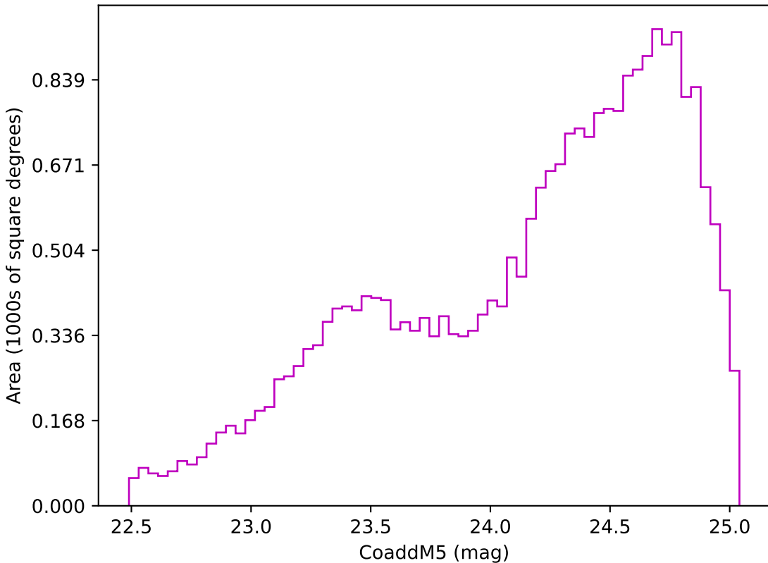
weather_cloudso10v3.4_10yrs Yr 3-4 z band: CoaddM5
