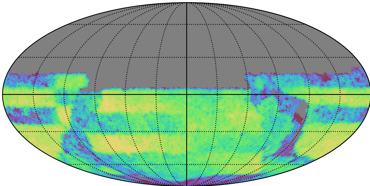
weather_cloudso10v3.4_10yrs Yr 3-4 y band: CoaddM5
