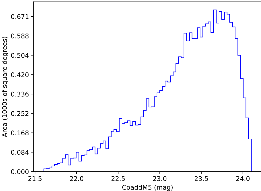
weather_cloudso10v3.4_10yrs Yr 3-4 y band: CoaddM5
