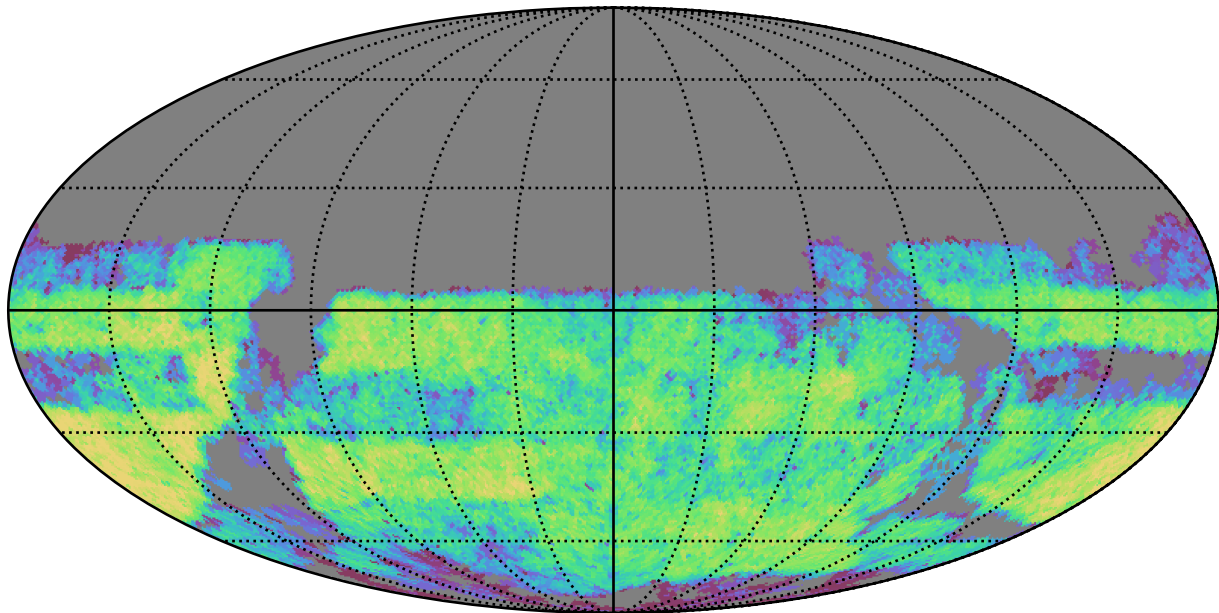
weather_cloudso10v3.4_10yrs Yr 3-4 u band: CoaddM5
