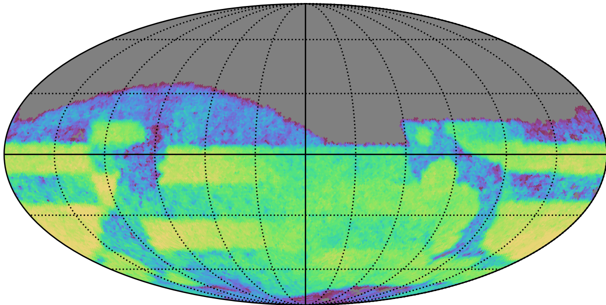
weather_cloudso10v3.4_10yrs Yr 3-4 r band: CoaddM5
