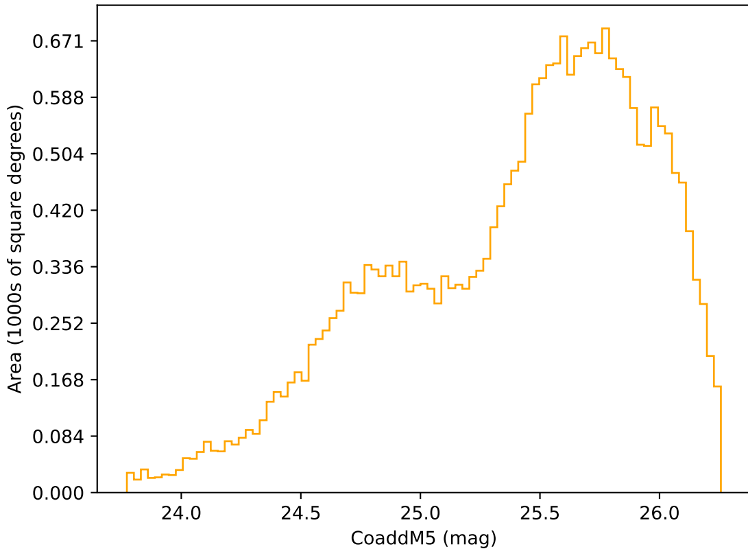
weather_cloudso10v3.4_10yrs Yr 3-4 r band: CoaddM5
