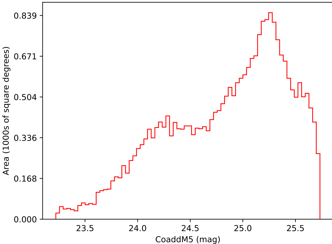
weather_cloudso10v3.4_10yrs Yr 3-4 i band: CoaddM5
