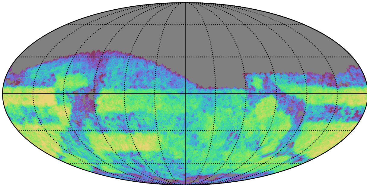
weather_cloudso10v3.4_10yrs Yr 3-4 g band: CoaddM5
