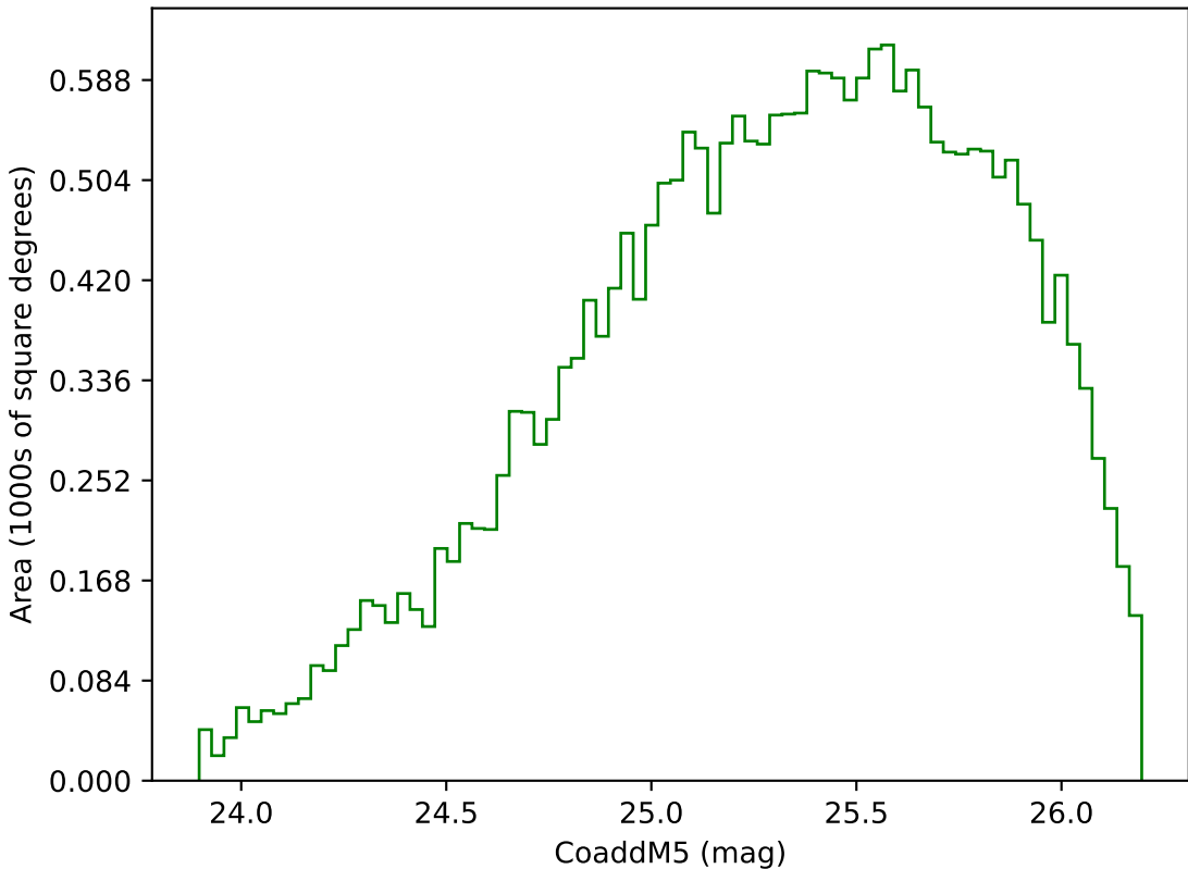
weather_cloudso10v3.4_10yrs Yr 3-4 g band: CoaddM5
