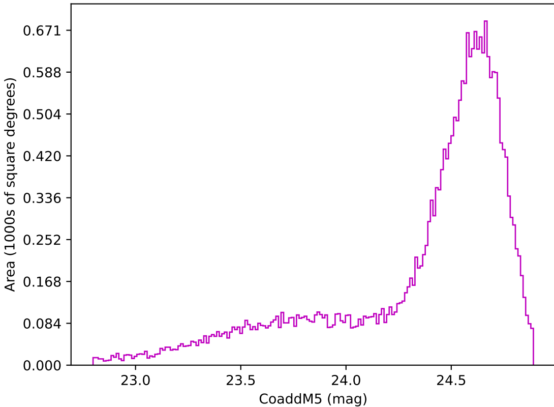
weather_cloudso10v3.4_10yrs Yr 1 z band: CoaddM5
