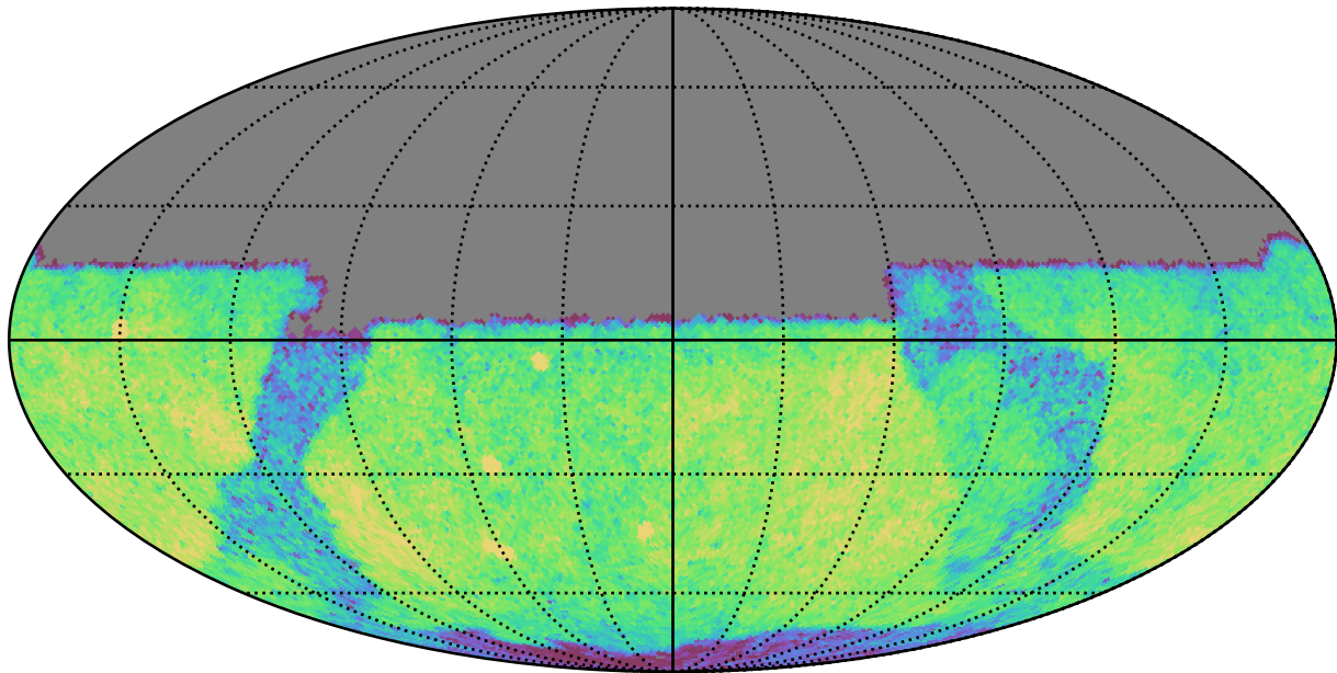
weather_cloudso10v3.4_10yrs Yr 1 y band: CoaddM5
