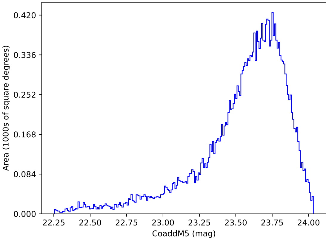
weather_cloudso10v3.4_10yrs Yr 1 y band: CoaddM5
