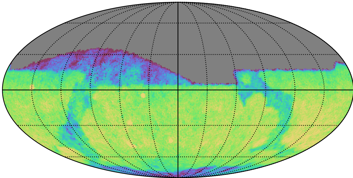
weather_cloudso10v3.4_10yrs Yr 1 r band: CoaddM5
