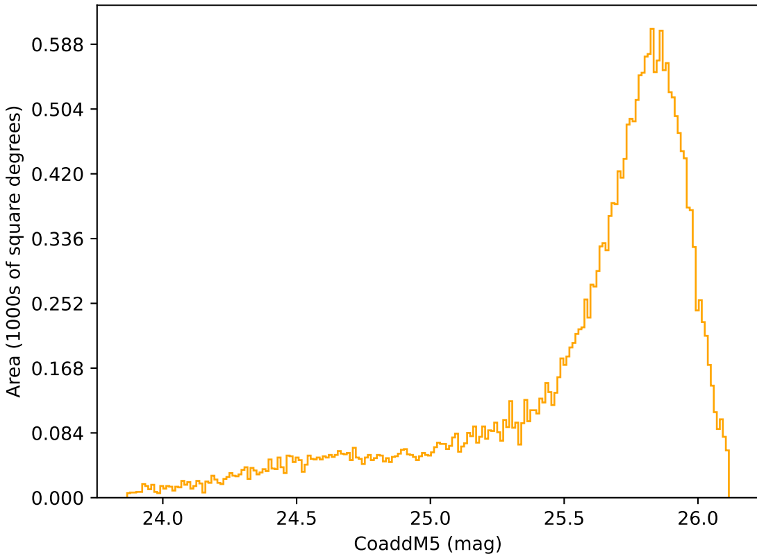
weather_cloudso10v3.4_10yrs Yr 1 r band: CoaddM5
