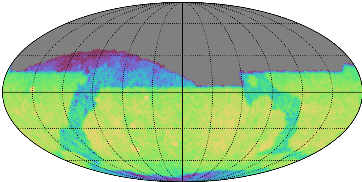
weather_cloudso10v3.4_10yrs Yr 1 i band: CoaddM5
