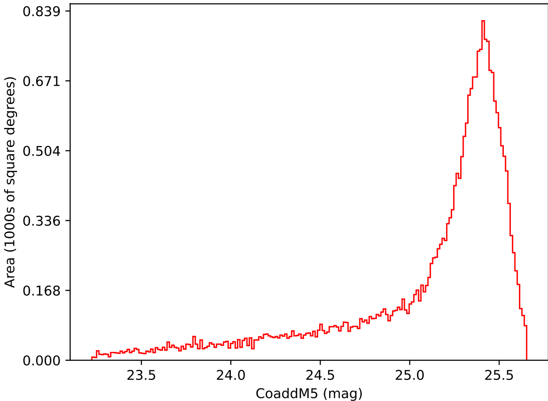
weather_cloudso10v3.4_10yrs Yr 1 i band: CoaddM5
