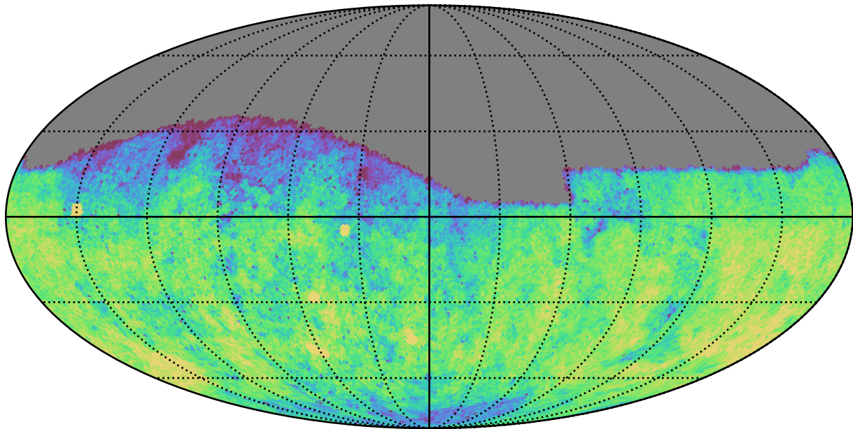
weather_cloudso10v3.4_10yrs Yr 1 g band: CoaddM5
