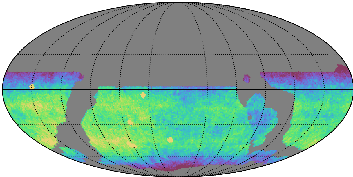
weather_cloudso10v3.4_10yrs WFD z band: CoaddM5
