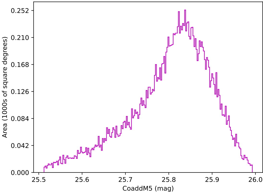
weather_cloudso10v3.4_10yrs WFD z band: CoaddM5
