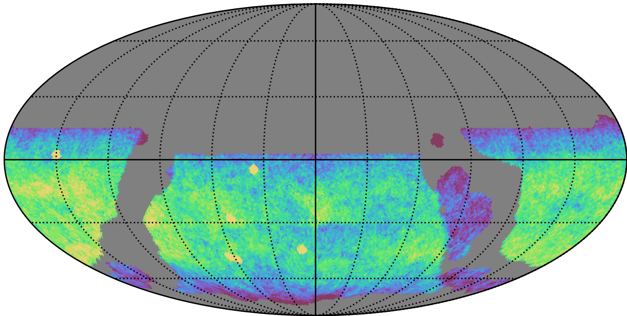
weather_cloudso10v3.4_10yrs WFD u band: CoaddM5
