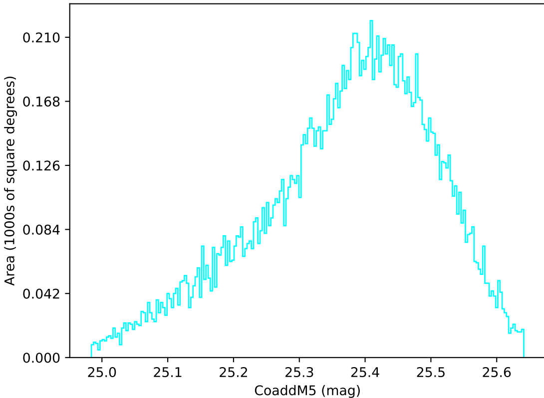
weather_cloudso10v3.4_10yrs WFD u band: CoaddM5
