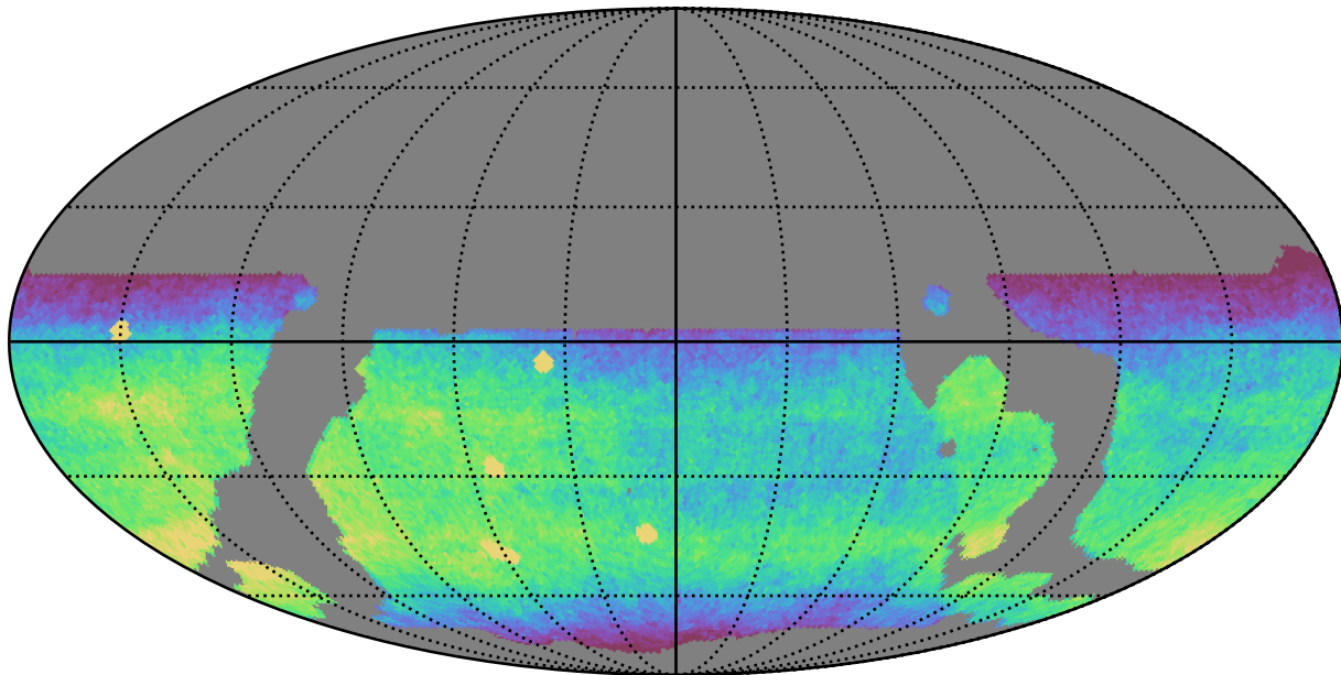
weather_cloudso10v3.4_10yrs WFD r band: CoaddM5
