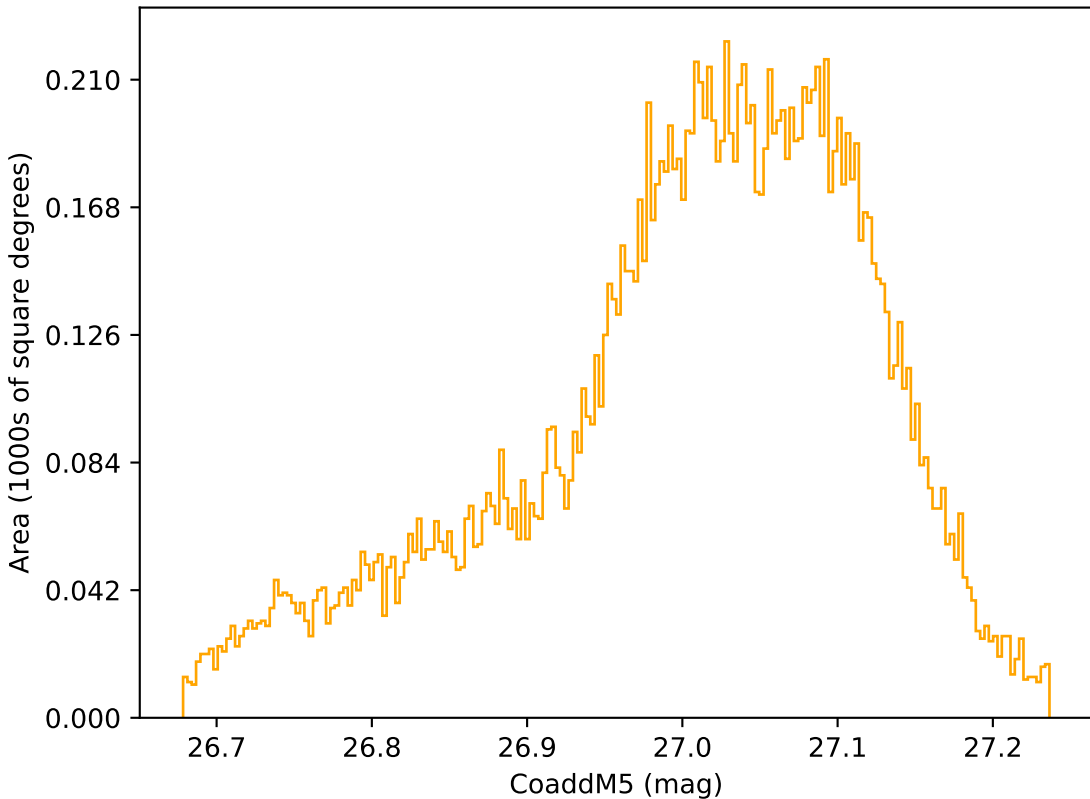
weather_cloudso10v3.4_10yrs WFD r band: CoaddM5
