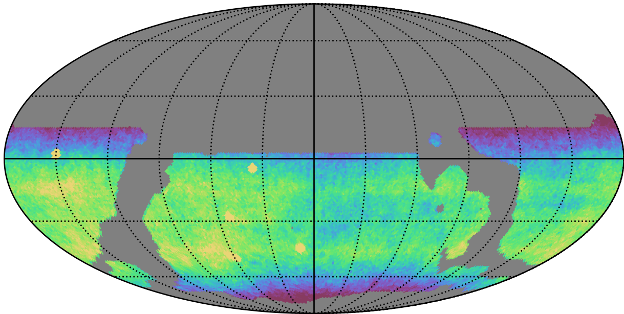
weather_cloudso10v3.4_10yrs WFD i band: CoaddM5
