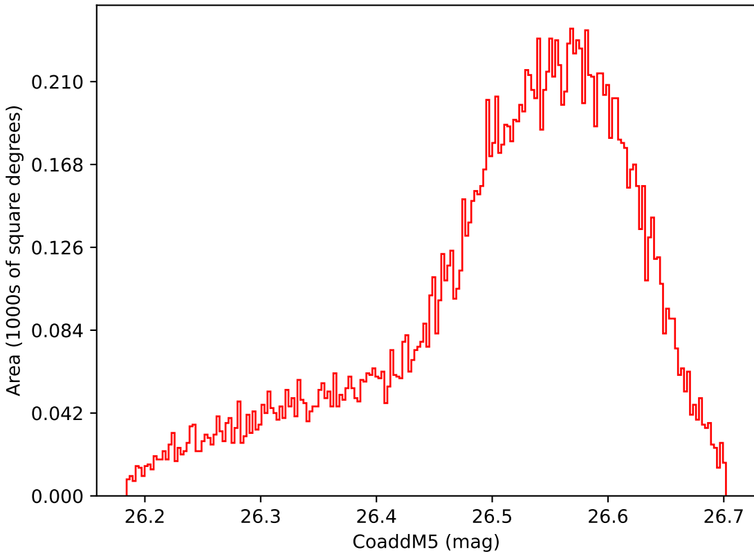
weather_cloudso10v3.4_10yrs WFD i band: CoaddM5
