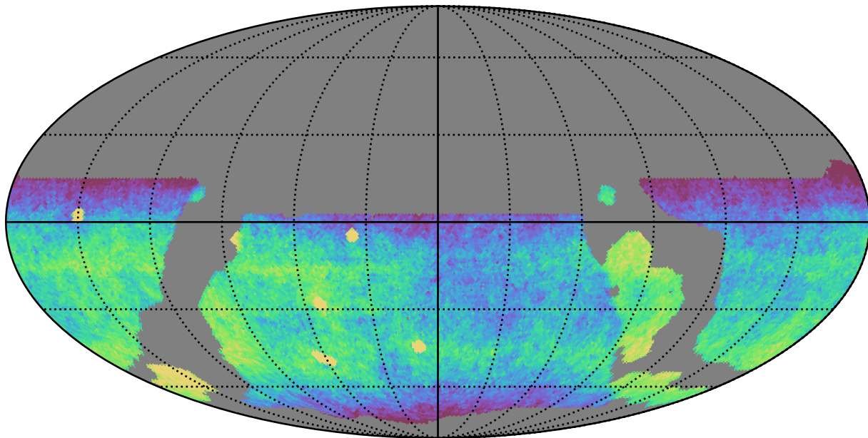
weather_cloudso10v3.4_10yrs WFD g band: CoaddM5
