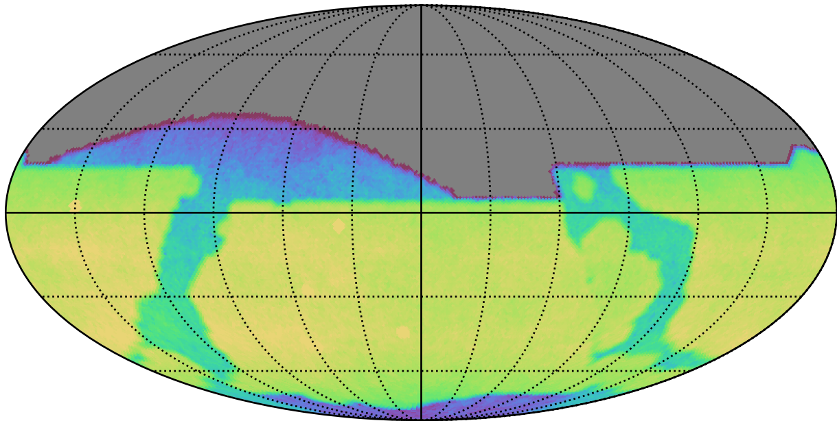
weather_cloudso10v3.4_10yrs All sky z band: CoaddM5
