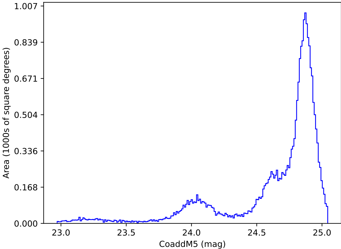
weather_cloudso10v3.4_10yrs All sky y band: CoaddM5
