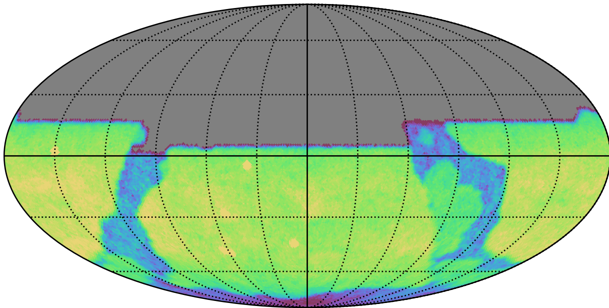
weather_cloudso10v3.4_10yrs All sky u band: CoaddM5
