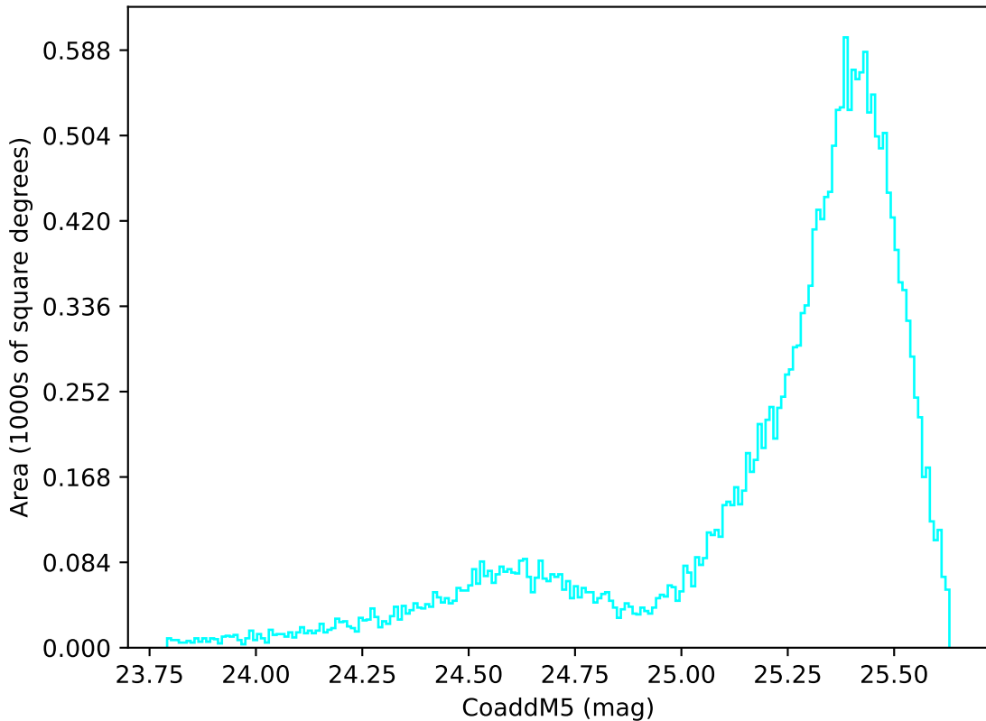
weather_cloudso10v3.4_10yrs All sky u band: CoaddM5
