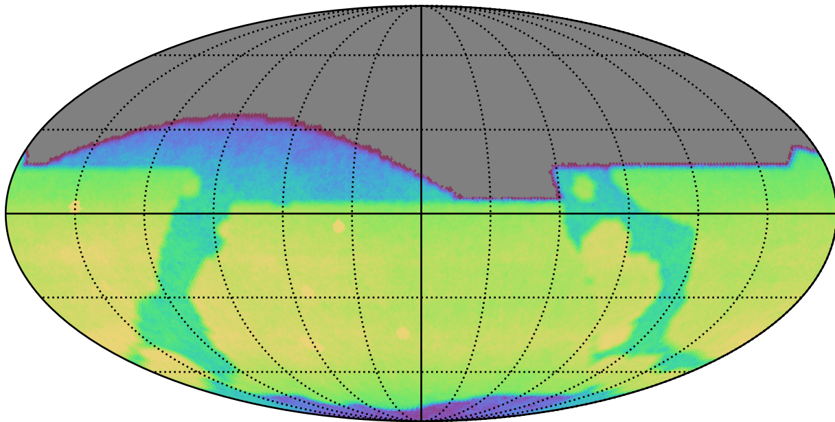
weather_cloudso10v3.4_10yrs All sky r band: CoaddM5
