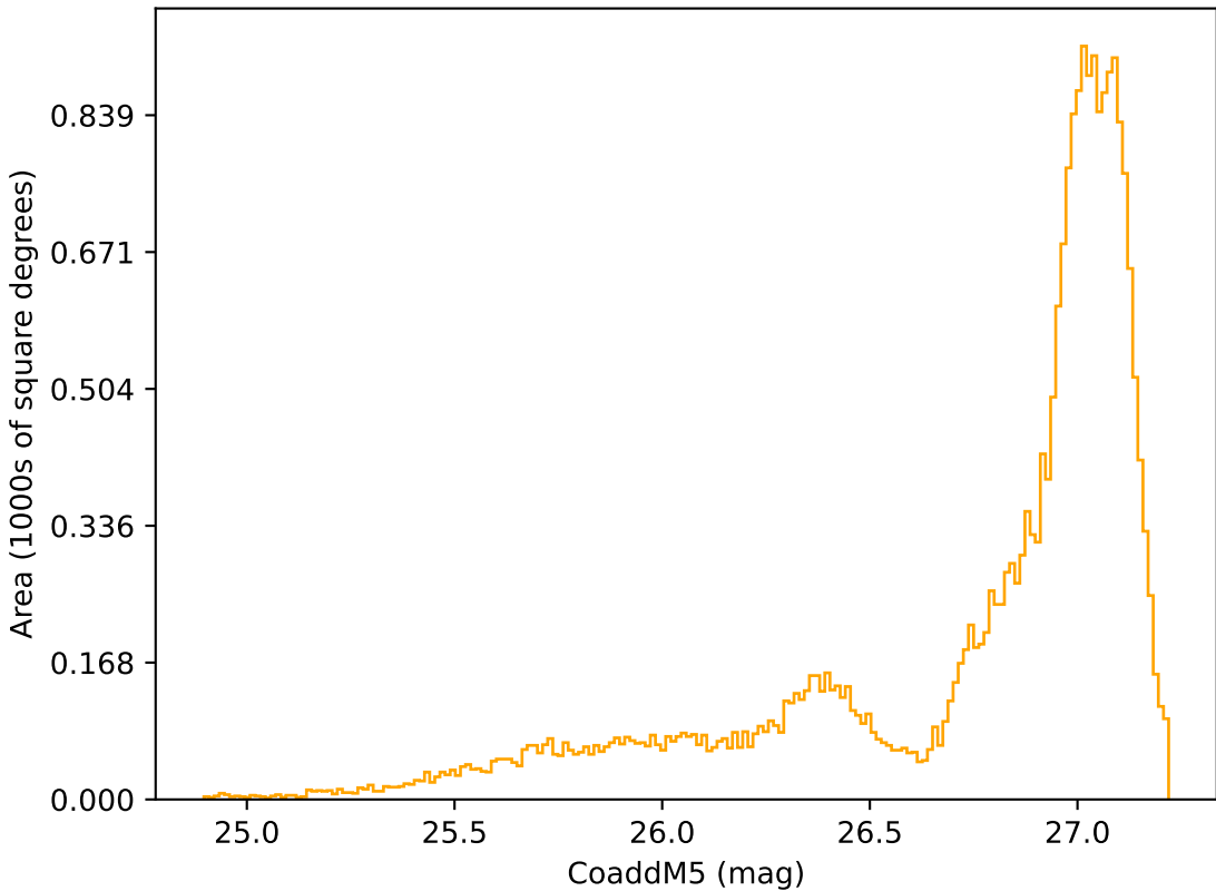
weather_cloudso10v3.4_10yrs All sky r band: CoaddM5
