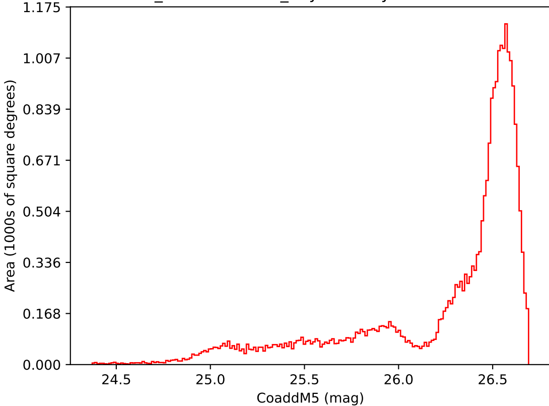
weather_cloudso10v3.4_10yrs All sky i band: CoaddM5
