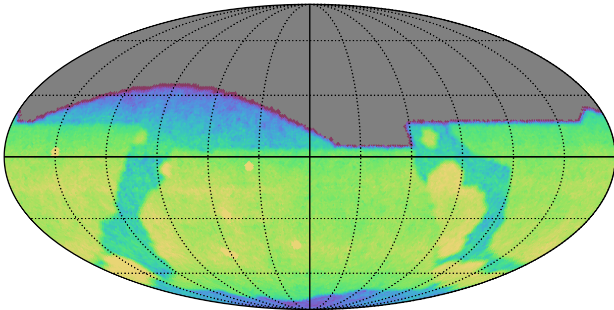
weather_cloudso10v3.4_10yrs All sky g band: CoaddM5
