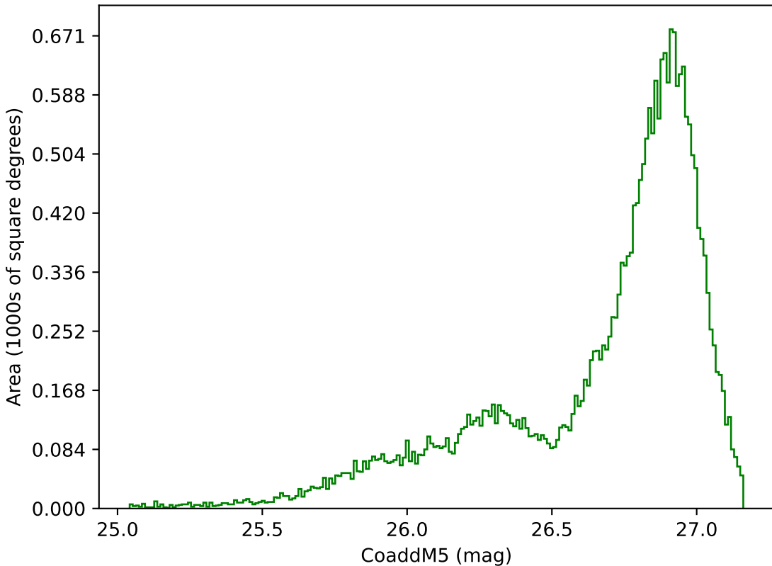
weather_cloudso10v3.4_10yrs All sky g band: CoaddM5
