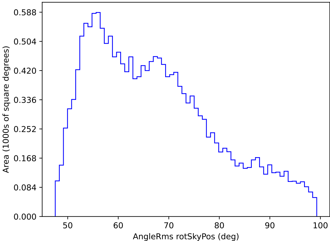
weather_cloudso10v3.4_10yrs WFD z band: AngleRms rotSkyPos
