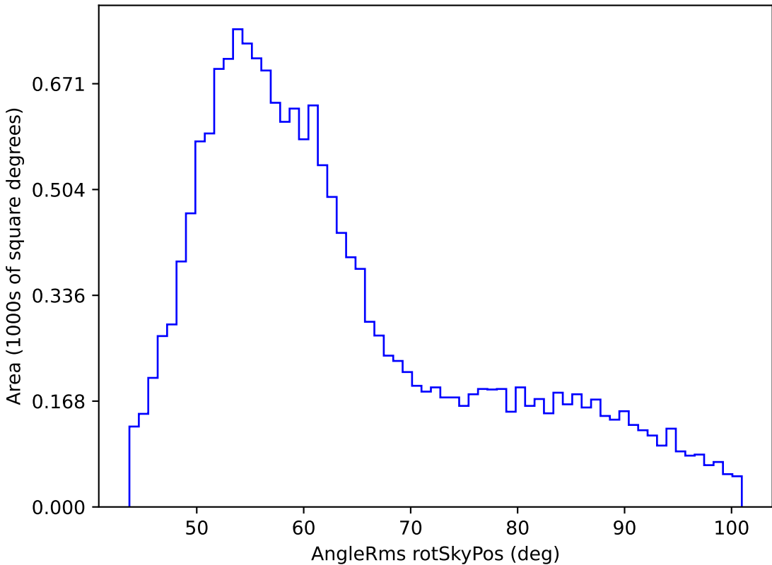
weather_cloudso10v3.4_10yrs WFD u band: AngleRms rotSkyPos
