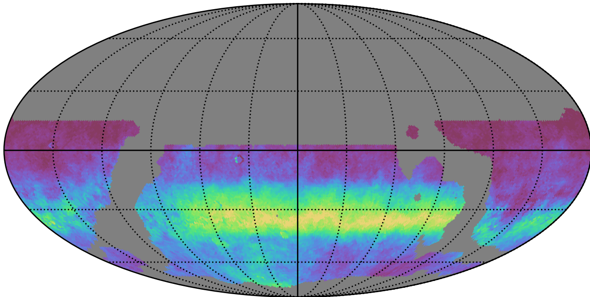
weather_cloudso10v3.4_10yrs WFD r band: AngleRms rotSkyPos
