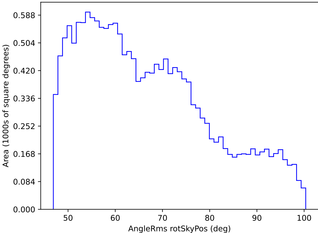
weather_cloudso10v3.4_10yrs WFD r band: AngleRms rotSkyPos
