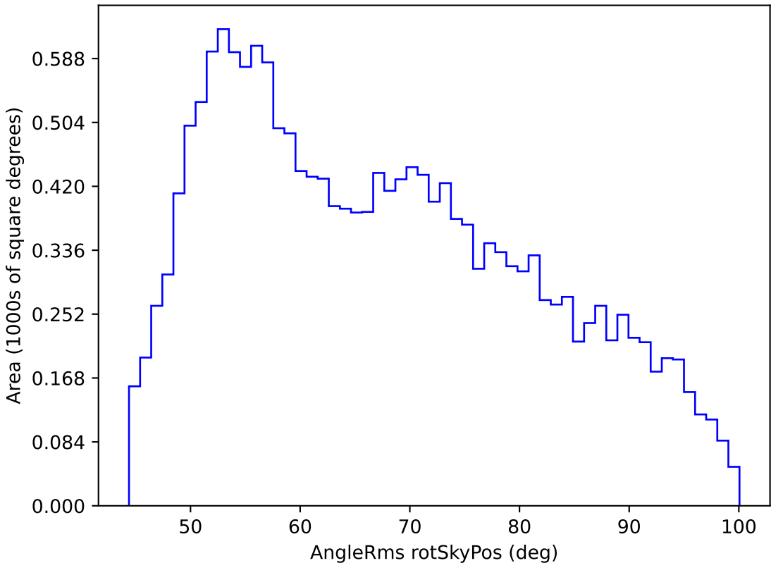
weather_cloudso10v3.4_10yrs WFD g band: AngleRms rotSkyPos
