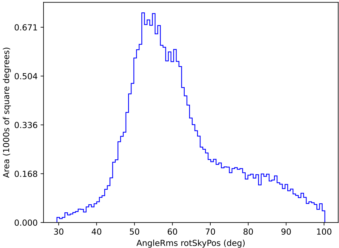
weather_cloudso10v3.4_10yrs All sky u band: AngleRms rotSkyPos
