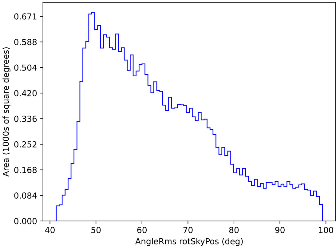
weather_cloudso10v3.4_10yrs All sky r band: AngleRms rotSkyPos
