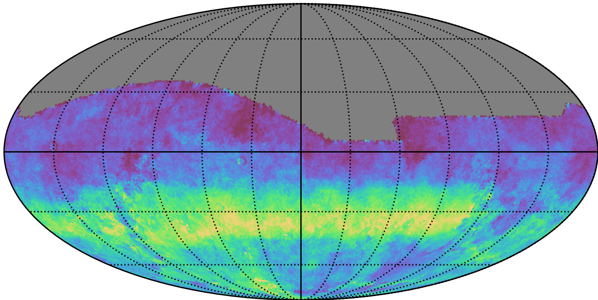
weather_cloudso10v3.4_10yrs All sky g band: AngleRms rotSkyPos
