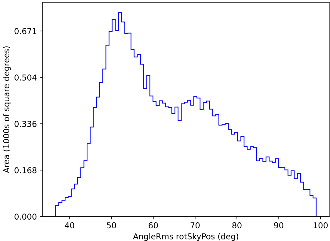
weather_cloudso10v3.4_10yrs All sky g band: AngleRms rotSkyPos
