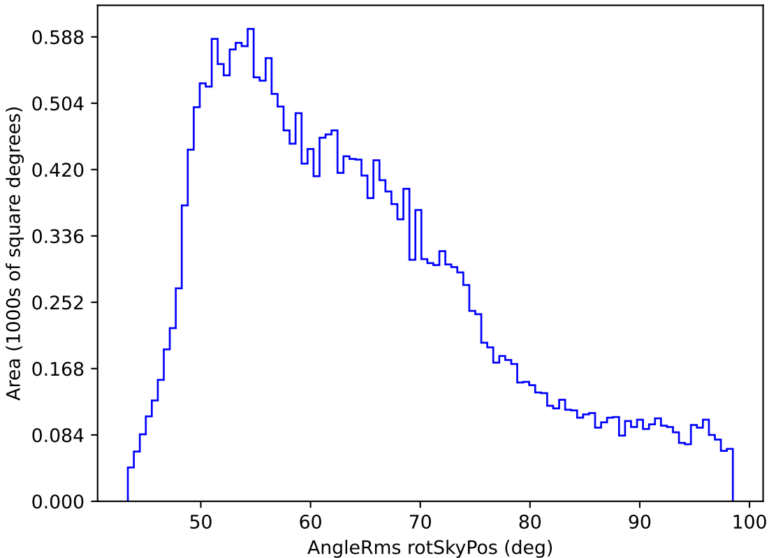
weather_cloudso10v3.4_10yrs All sky all bands: AngleRms rotSkyPos
