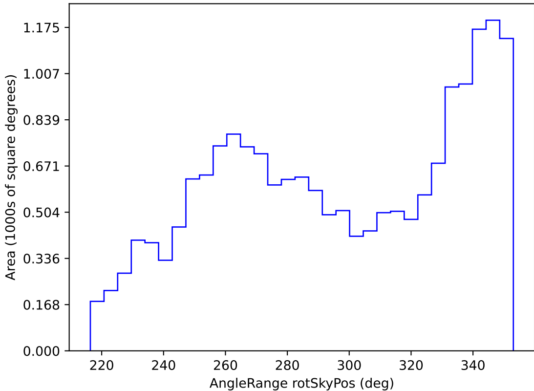
weather_cloudso10v3.4_10yrs WFD all bands: AngleRange rotSkyPos
