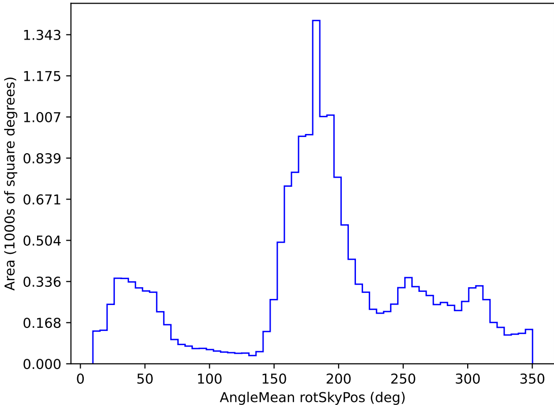
weather_cloudso10v3.4_10yrs WFD u band: AngleMean rotSkyPos
